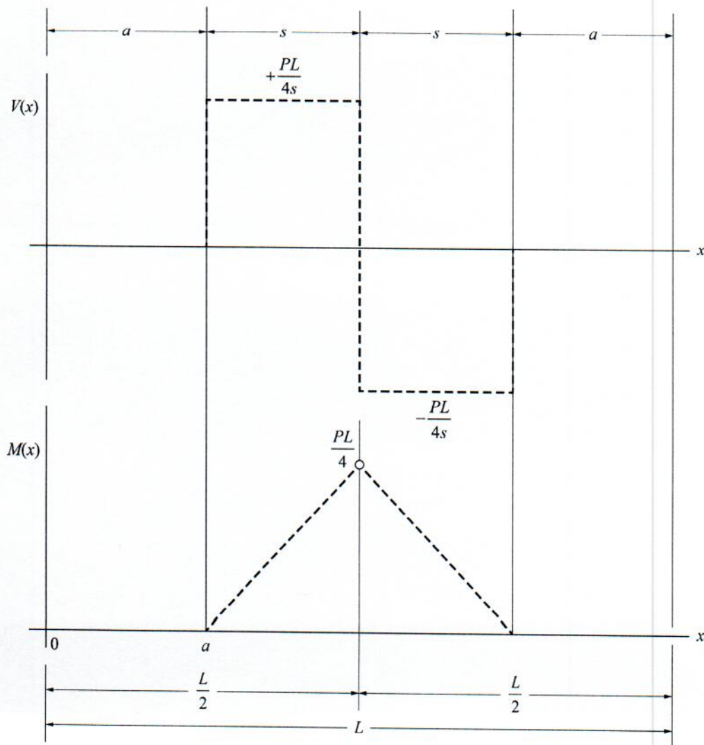
Shear and bending moment diagrams for Anderson splice
